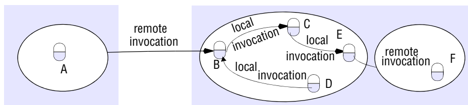
Figure 5.12 Remote and local method invocations
