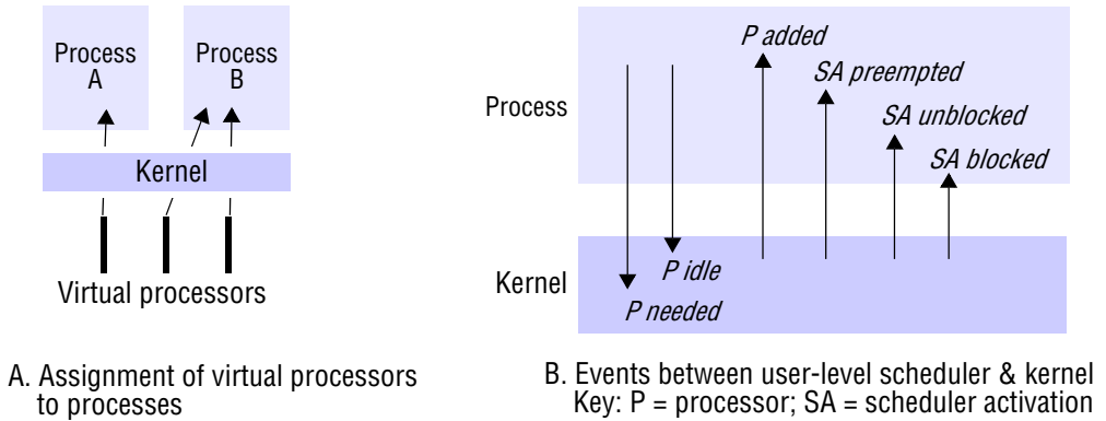
Figure 7.10 Scheduler activations
