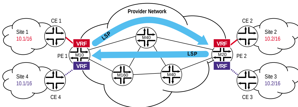
Figure 3: LSPs Between Site 1 and Site 2
