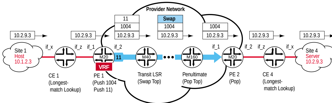
Figure 14: Forwarding VPN Red Traffic from Site 1 to Site 4
